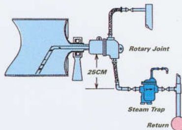
Fig. 8 A REVOLVING CYLINDER DRAINED WITH A SIPHON
