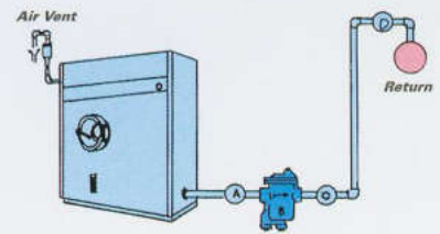
Fig. 3 POSSIBLE CHECK VALVE LOCATION
