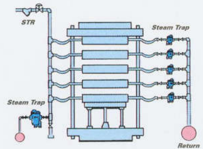
Fig. 6 PRODUCT CONFINED IN STEAM JACKETED PRESS
