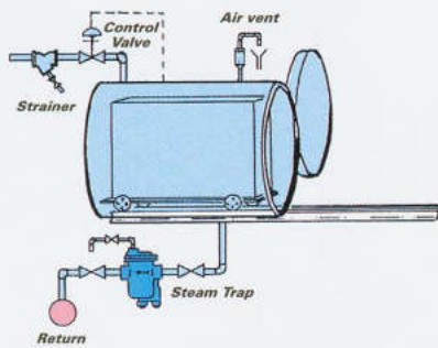
Fig. 5 DIRECT STEAM INJECTION INTO PRODUCT CHAMBER
