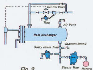
Fig. 9 SHELL AND TUBE HEAT EXCHANGERS
