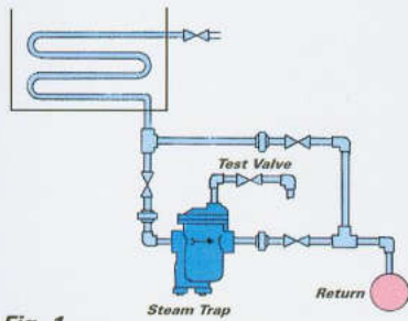
Fig. 1 TYPICAL NICOLSON STEAM TRAP BYPASS HOOK UP
