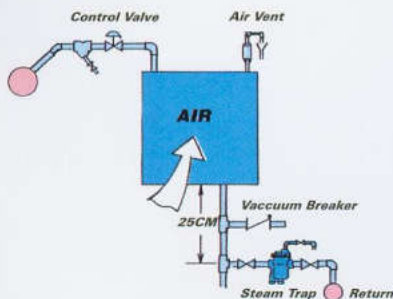
Fig. 7 TRAPPING AND VENTING AIR HEAT COIL
